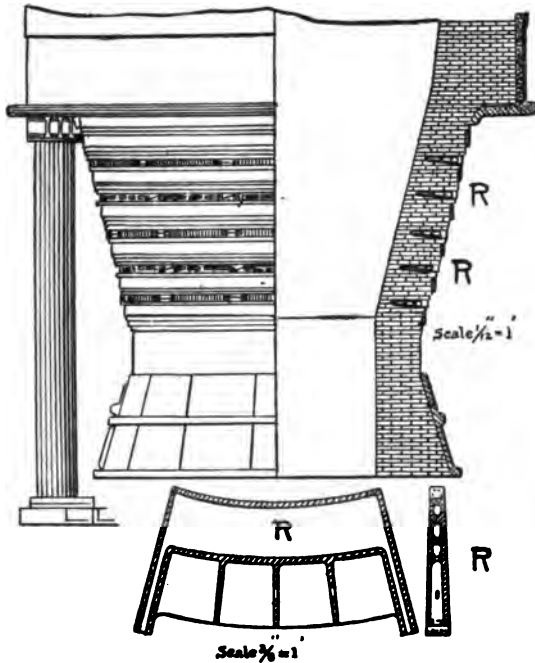
Fig. 92. Gayley's Water-cooling Blocks for Cooling the Inner Face of the Walls of Blast-furnaces.
